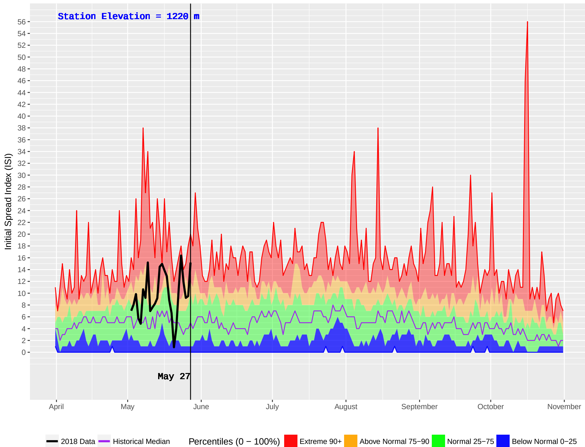
NEMIAH (216) : Historical (1982–2016) and Current (2018) Noon Initial Spread Index (ISI)
