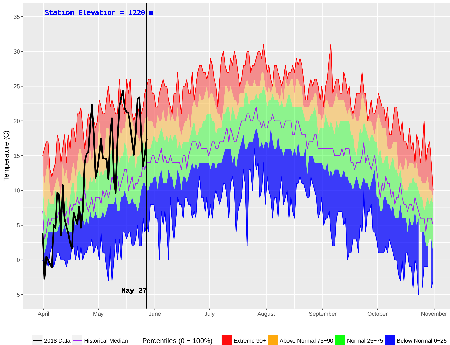
NEMIAH (216) : Historical (1982–2016) and Current (2018) Noon Temperature
